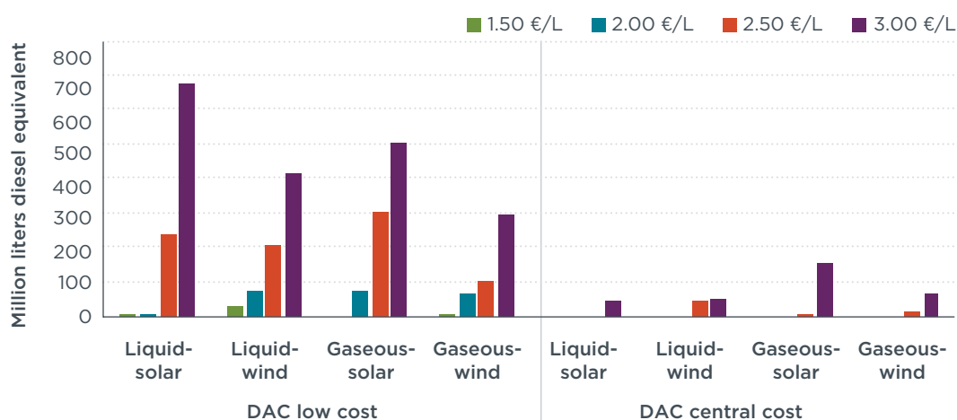
Figure 5. Total EU electrofuel potential in 2030 in Scenario 2 (grid-connected) with DAC CO 2 (million liters diesel equivalent).
